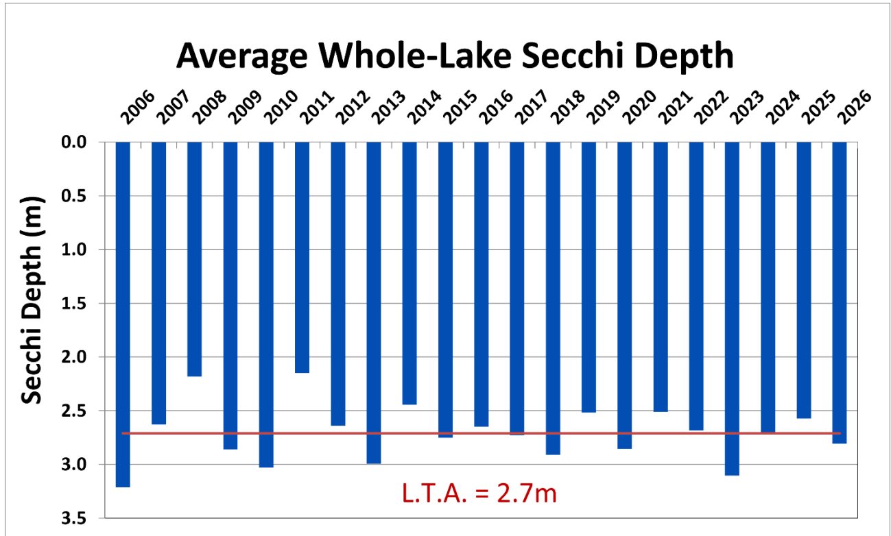
Figure 3: Whole-Lake Secchi Depth average by year. The red line indicates the 21-year LTA of 2.7 m.
