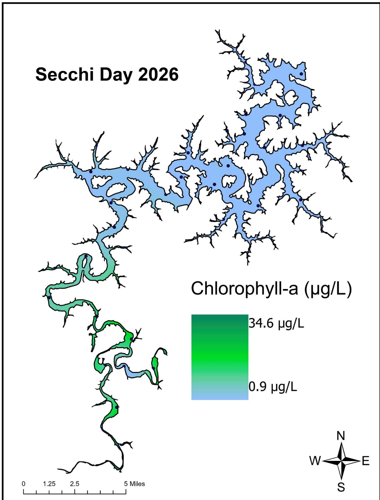
Figure 2: Chlorophyll-a concentrations ranged from 0.92 \mu\text{g/L} to 34.61 \mu\text{g/L} .
