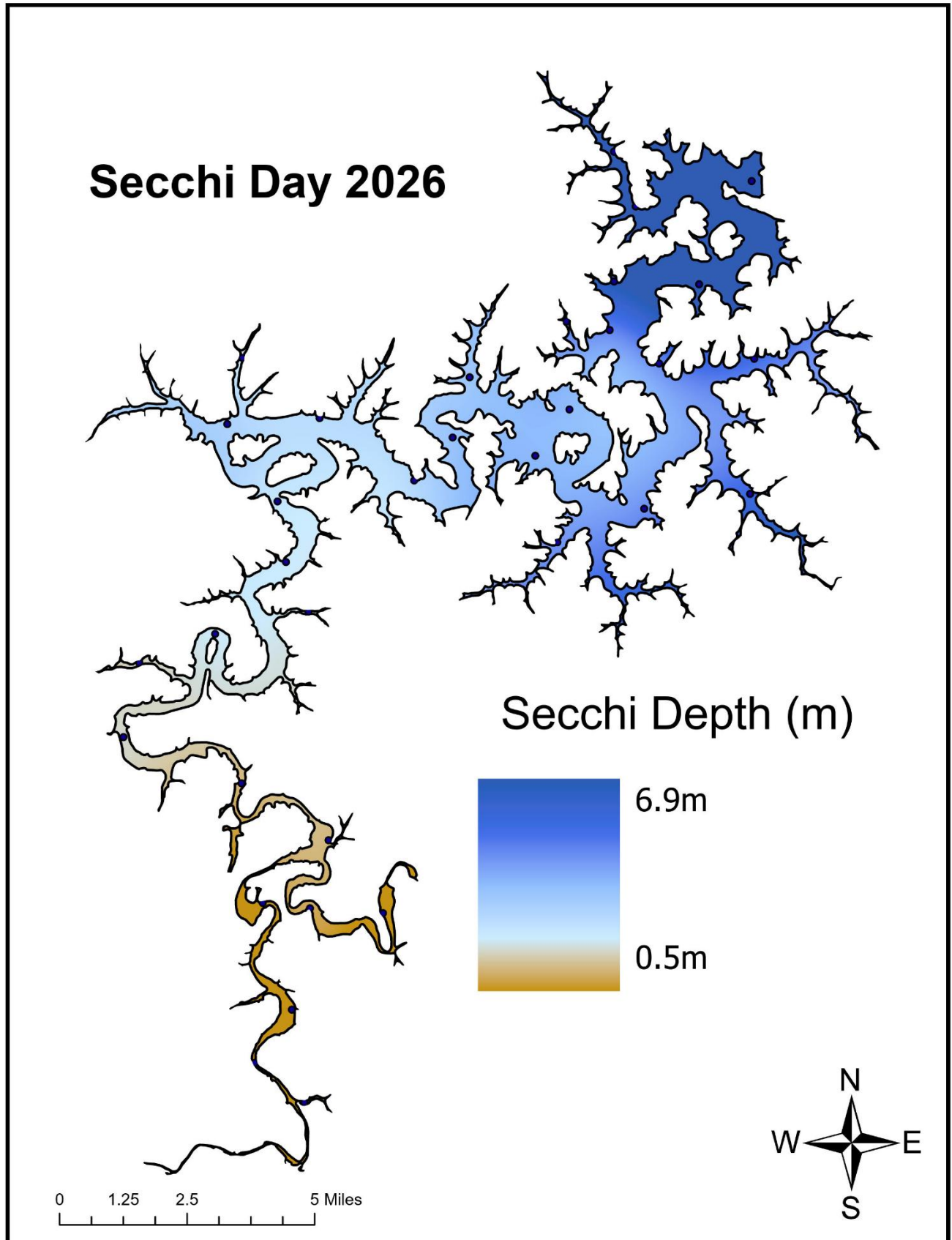
Figure 1: Secchi Depths ranged from 0.5 meters to 6.9 meters.
