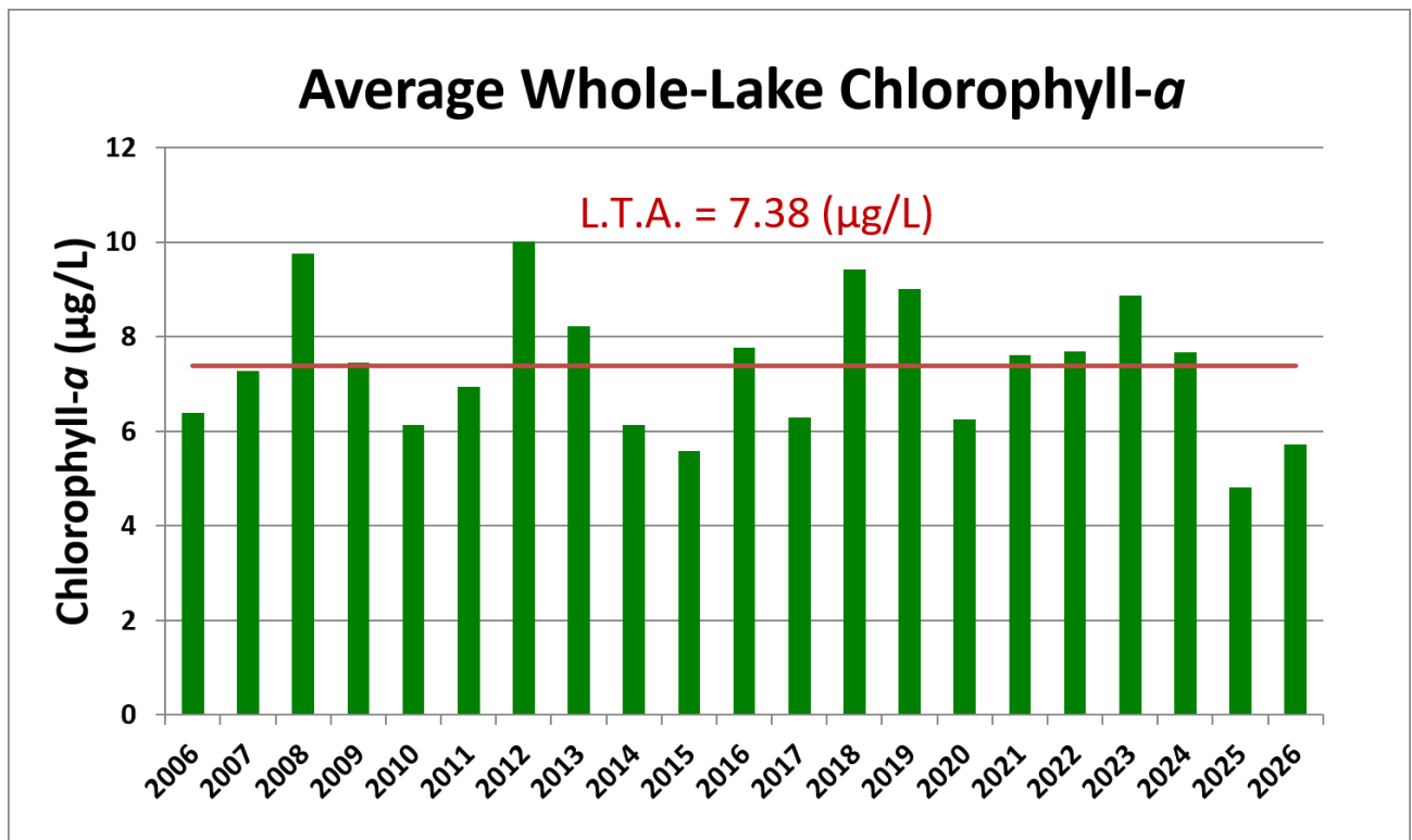
Figure 4: Whole-Lake Chlorophyll-a average by year. The red line indicates the 21-year LTA of 7.38 µg/L.
